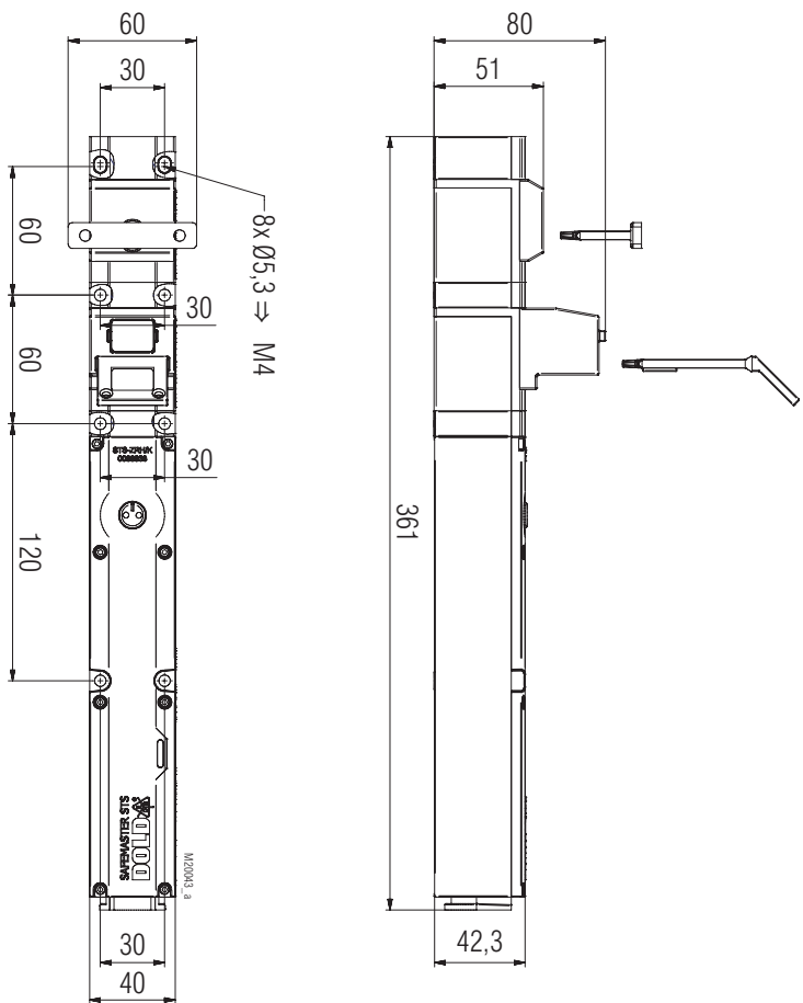
ZRH01BM/K Clearance tolerances ± 2%
