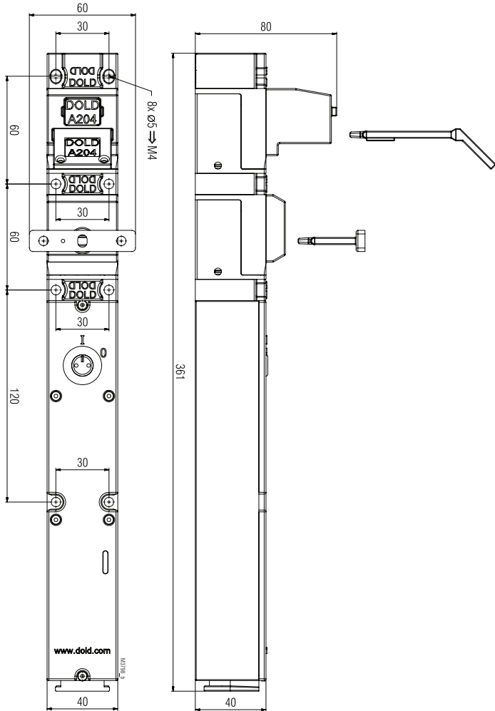
ZRHB01M/K Clearance tolerances \pm 2\%
