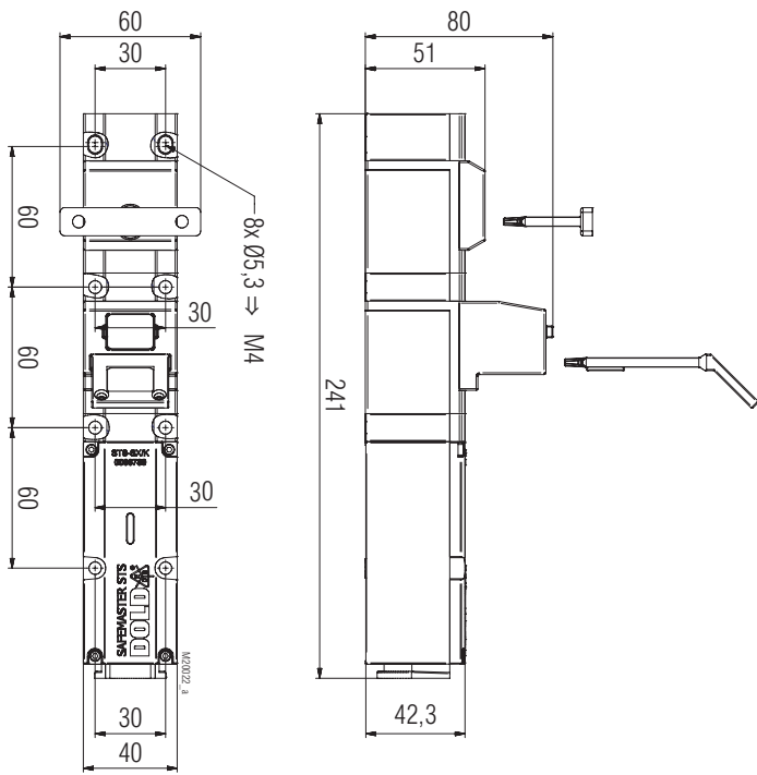
SX01BM/K Clearance tolerances ± 2%
